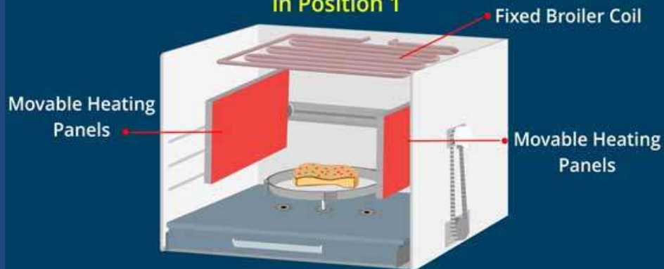
Movable Heating Panels in Position 1
